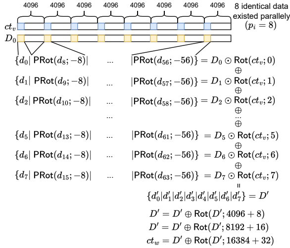
Figure 11: A simple illustration of parallel BSGS diagonal method.
