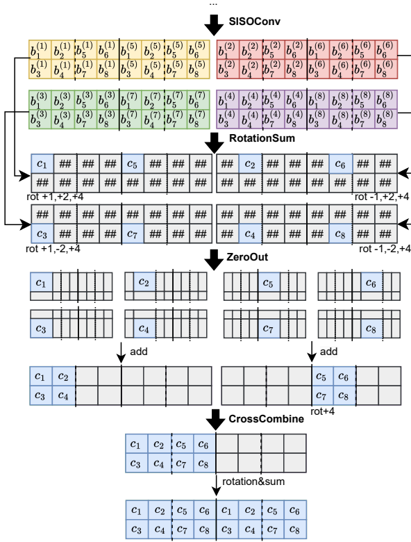
Figure 5: A conceptual diagram of the high-level idea of RO-MPCov, under the same conditions as in Figure 3.
