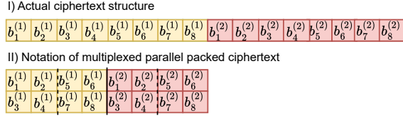
Figure 2: Notation of multiplexed parallel packed ciphertext in this paper.
