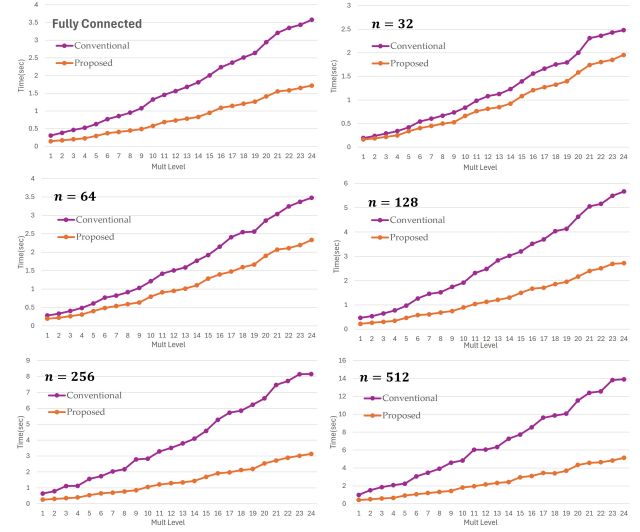
Figure 15: Latency comparison of parallel BSGS matrix-vector multiplication and BSGS diagonal method.
