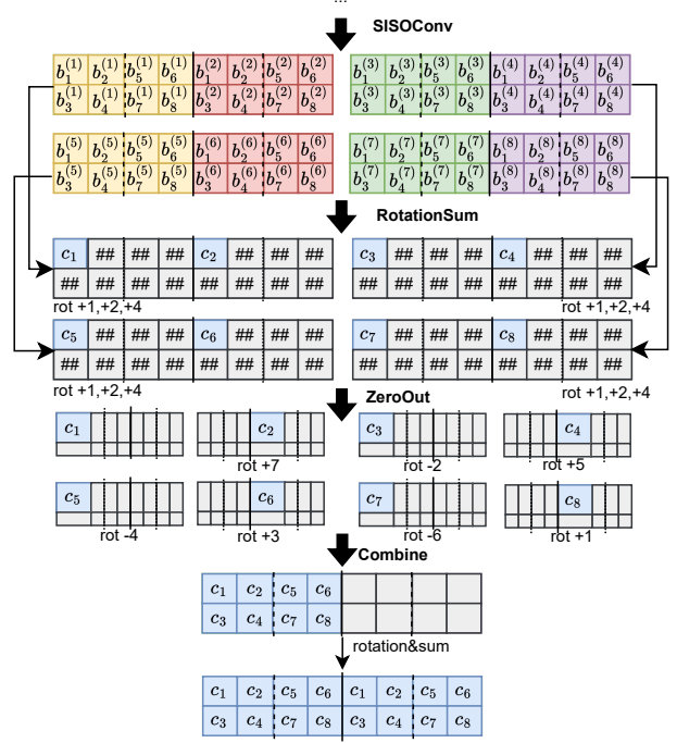
Figure 3: A conceptual diagram example of MPCConv [8] where w_i = h_i = w_o = h_o = 1 , f_w = f_h = 3 , c_i = c_o = 8 , p_i = p_o = 2 , k_i = k_o = 2 .
