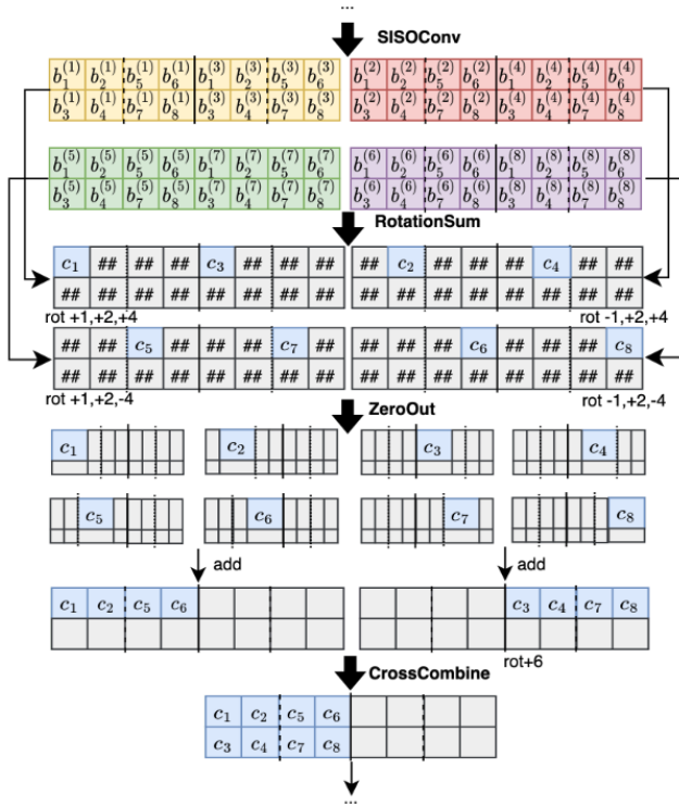
Figure 8: Showing the non-uniqueness property of RO-MPConv. Same condition, and same performance as Figure 5, but the kernel arrangement and shift amount of rotation are different.
