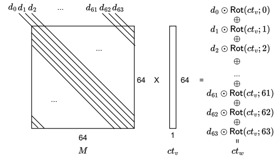
Figure 9: A simple illustration of diagonal method([12]) for matrix-vector multiplication.
