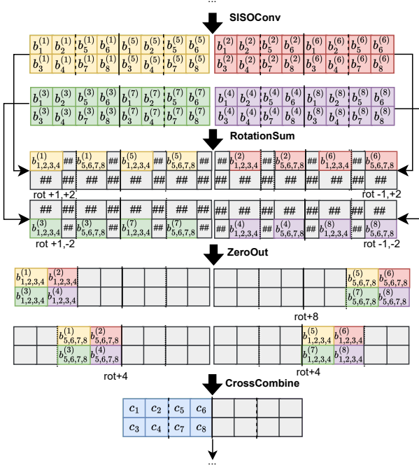
Figure 6: A conceptual diagram showing how RO-MPConv leverages the correlation between the RotationSum and CrossCombine stages to reduce rotation counts.
