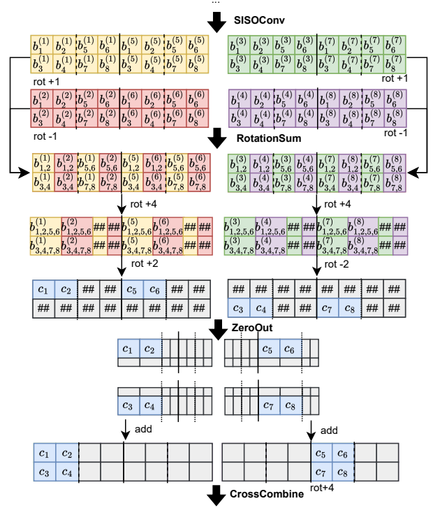
Figure 7: A conceptual diagram of the RO-MPConv variant that utilizes an additional multiplicative depth.
