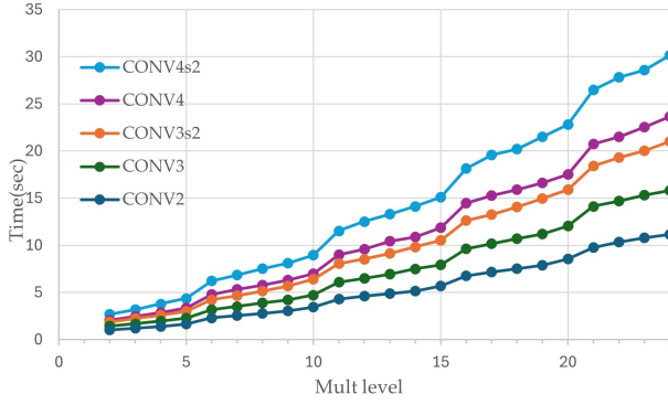
Figure 4: Latency of MPConv in various multiplication levels.
