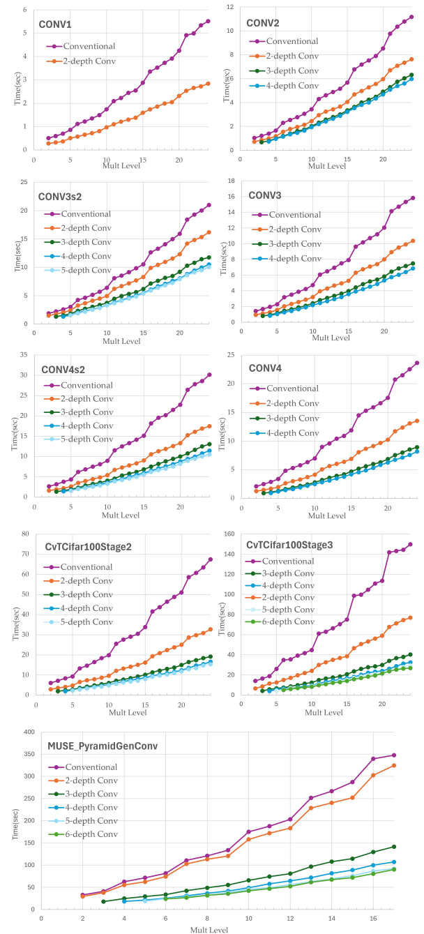
Figure 13: Latency comparison of proposed (ROMPConv) and conventional (multiplexed parallel convolution in [8]) convolution. For MuseConv, we used a lighter CKKS parameter setting with \log Q = [51, 41, 40, 40, 41, 40, 41, 40, 40, 40, 41, 41, 40, 41, 40, 40, 40] and \log P = [50, 51, 50] due to memory constraints.
