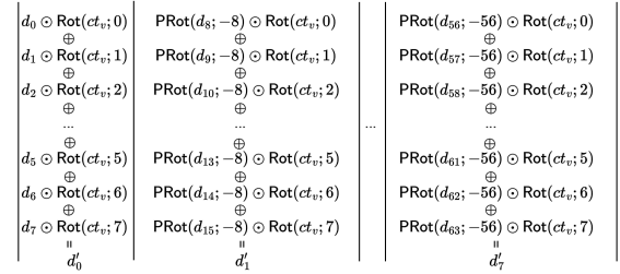
Figure 9: A simple illustration of diagonal method([12]) for matrix-vector multiplication.
