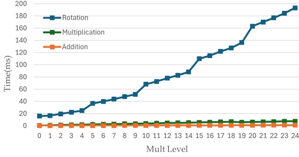
Figure 1: Latency of RNS-CKKS basic operation - addition, plaintext multiplication, rotation.
