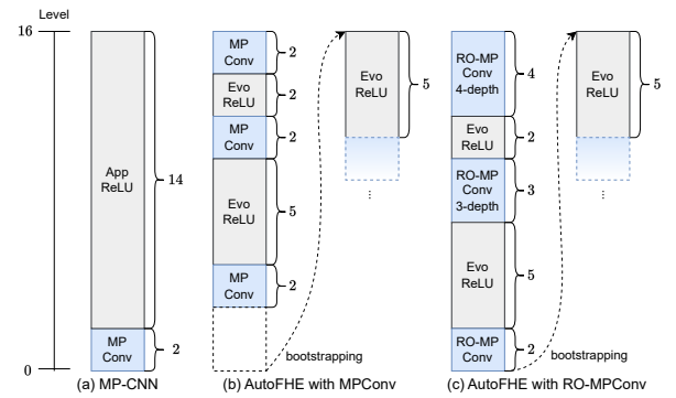
Figure 14: Comparison of operational layouts across multiplicative levels in different model architectures. (a) The baseline MP-CNN, which utilizes a deep polynomial activation (AppReLU), requiring MPConv operations to be scheduled at the lowest (fastest) levels immediately before bootstrapping. (b) AutoFHE with standard MPConv, where the use of mixed-degree activations (EvoReLU) results in convolutions being scheduled at higher levels and creates intermittent unused level gaps. (c) Our proposed application, where MPConv is replaced by RO-MPConv. By employing RO-MPConv variants with additional depth (e.g., 3-depth, 4-depth), we can efficiently schedule operations to fill these previously wasted levels, creating an optimized computational graph and reducing overall latency.
